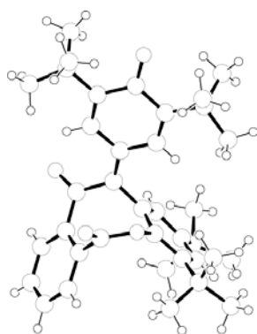
Figure 1. X-ray structure of 5 .
