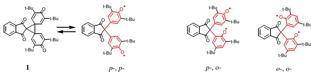
Scheme 1. Isomeric diradicals based on bis(hydroxyphenyl)methane.
