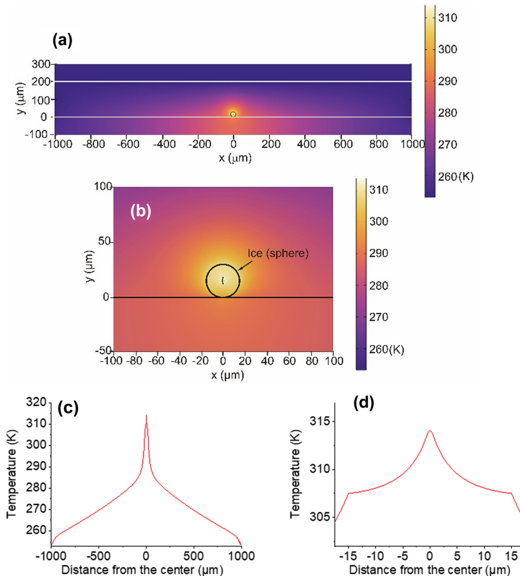
Fig. 8 Temperature distribution in a sample chamber (formed by the space between two glass substrates separated by a 200 \mu\text{m} spacer) during illumination with a 1064-nm laser (50 mW). (a) Ice particle of diam. = 30 \mu\text{m} supported on a substrate. (b) Expanded image of (a). (c) 1D temperature distribution on the equator in the horizontal direction. (d) Horizontal expansion from the graph in (c). The chamber wall temperature was fixed at -20\text{ }^{\circ}\text{C} (253 K).
