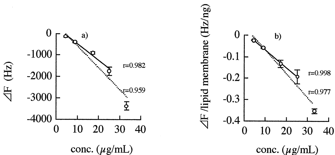
Fig. 12 Relation between frequency changes of quartz crystal microbalance and indomethacin concentration in 10% ethanol
