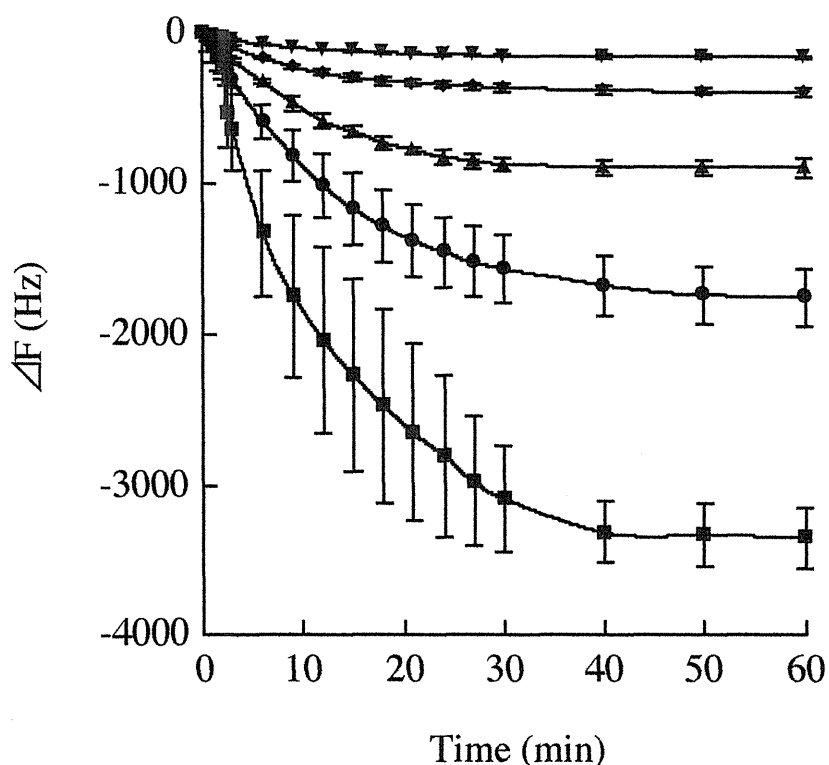
Fig. 9 Time course of change in frequency decrease in indomethacin in 10% ethanol measured by quartz crystal microbalance
