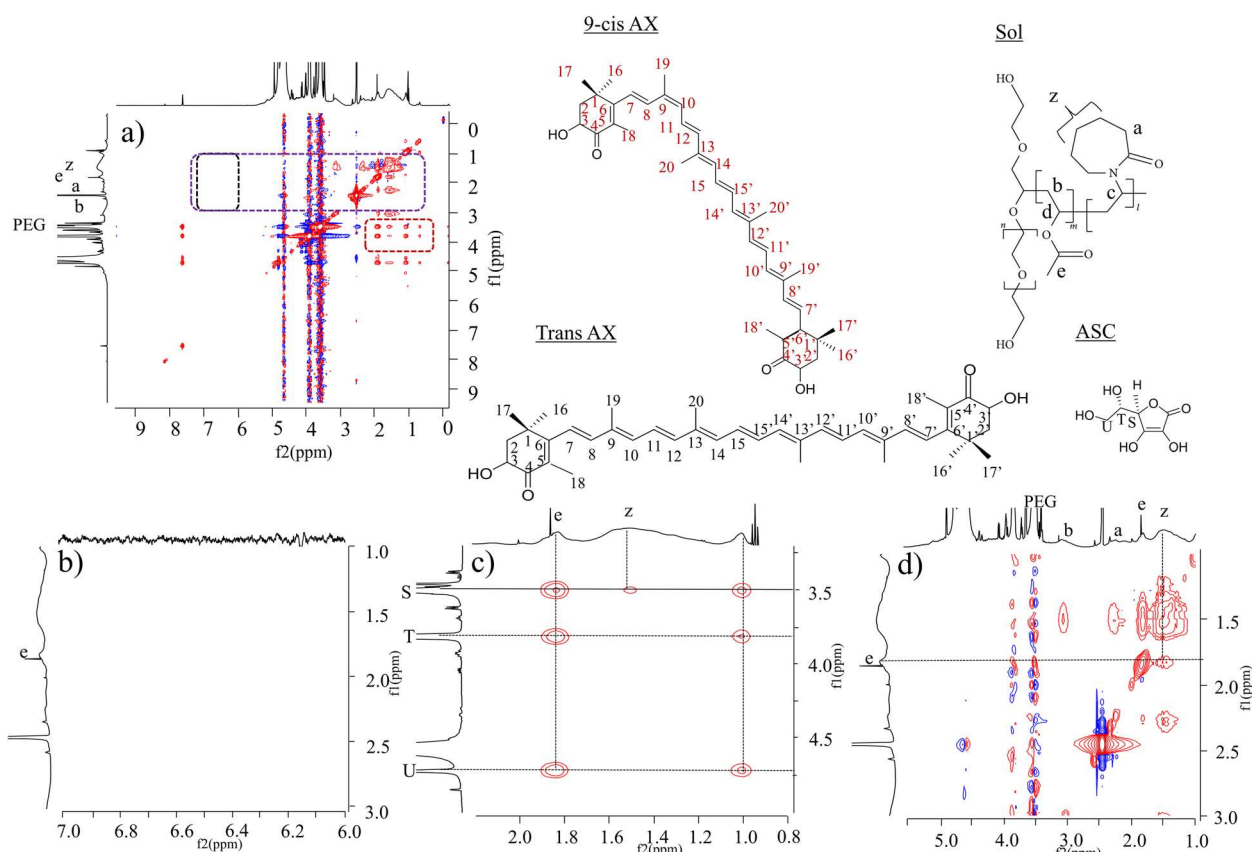
Fig. 10 ^1\text{H} - ^1\text{H} NOESY NMR spectra of EVP (Sol/AX=9/1) in 0.1 M ASC+DMSO. a f1 is 0–9 ppm, f2 is 0–9 ppm, b f1 is 6–7 ppm, f2 is 1–3 ppm, c f1 is 4–7 ppm, f2 is 2.8–3–3.8 ppm, d f1 is 1–7 ppm, f2 is 1–3 ppm
