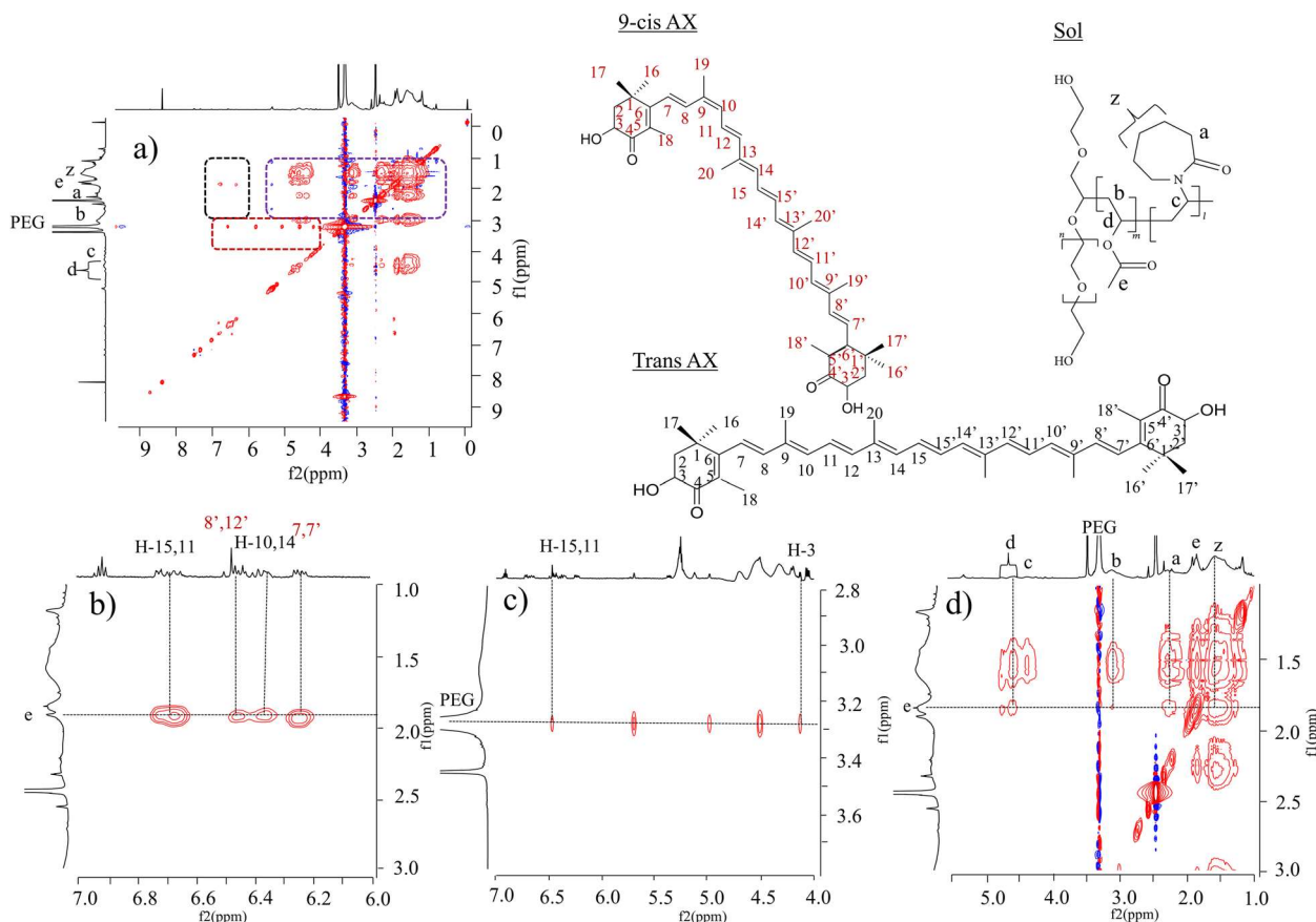
Fig. 9 ^1\text{H} - ^1\text{H} NOESY NMR spectra of EVP (Sol/AX=9/1) in \text{DMSO-d}_6 . a f_1 is 0–9 ppm, f_2 is 0–9 ppm, b f_1 is 6–7 ppm, f_2 is 1–3 ppm, c f_1 is 4–7 ppm, f_2 is 2.8–3.3 ppm, d f_1 is 1–7 ppm, f_2 is 1–3 ppm
